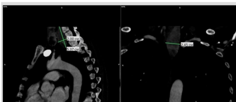
Figure 1. Spiral CT of the neck and upper mediastinum
