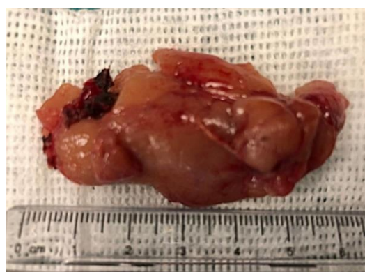
Figure 5. Parathyroid adenoma 7 x 3 x 1,5 cm
