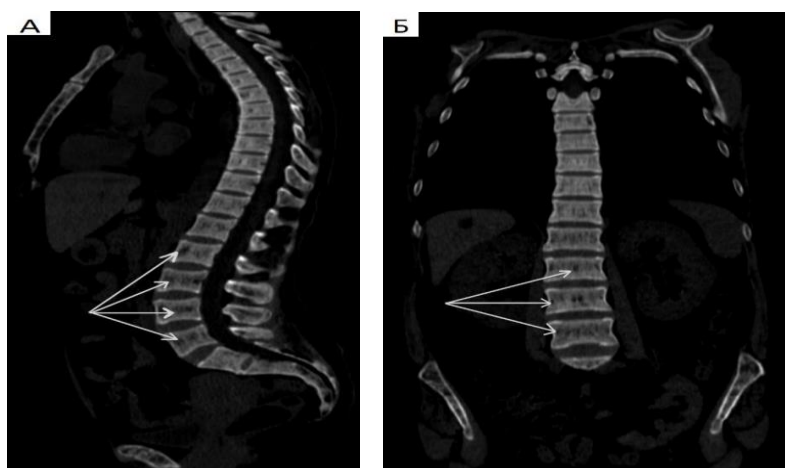
Figure 2. CT of the spine. Sagittal (A) and coronal (B) reconstructions. Signs of osteoporosis (indicated by arrows)
